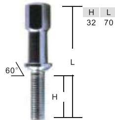
WB011 17mm HEX ø22mm
