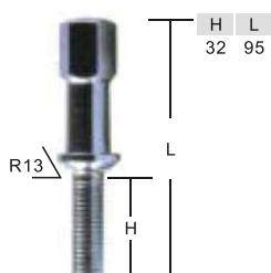
WB015 17mm HEX ø21.5mm
