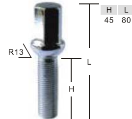
WB008 17mm HEX
