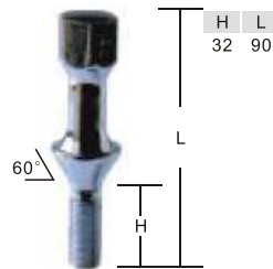
WB012 19mm HEX ø21.5mm
