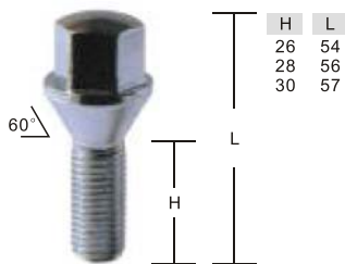
WB001 17mm HEX Ø23mm
